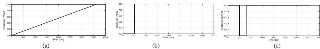
Figure 4- Unsteady input conditions – (a) Ramp, (b) step and (c) valley test cases.
